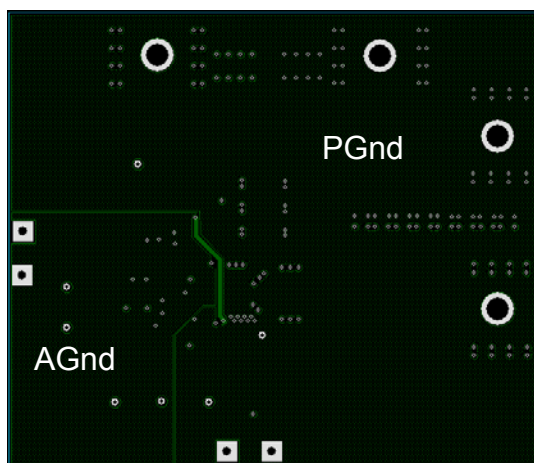
Fig. 28c. IRDC3853 demoboard layout considerations – Mid Layer 1
