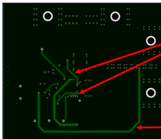
Fig. 28d. IRDC3853 demoboard layout considerations – Mid Layer 2
